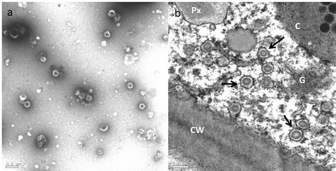
Fig. 3 Transmission electron micrographs of Groundnut ringspot tospovirus (GRSV) in infected petunia ( Petunia hybrida ) leaves. a Negatively stained leaf extract, showing a group of presumed membrane-bounded GRSV virions, with circular profile ca. 100 nm in
