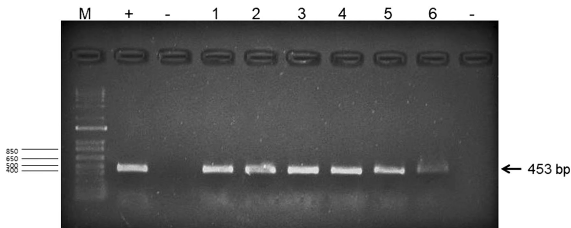
Fig. 2 Agarose gel showing the results of the detection of Groundnut ringspot tospovirus by RT-PCR in tomato ( Solanum lycopersicum ) (1–3) and petunia ( Petunia hybrida ) (4–6) samples. +: control infected with GRSV, -: healthy controls
